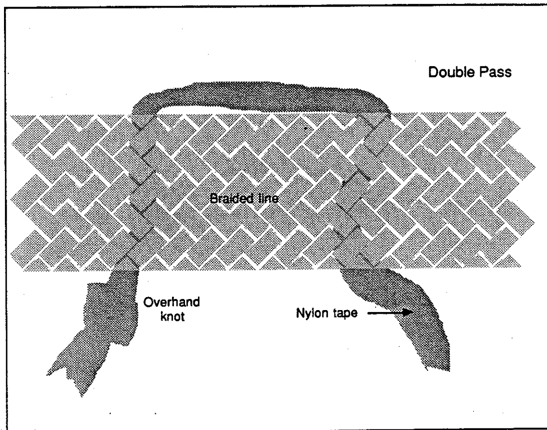
FIGURE 18. Splicing Methods
