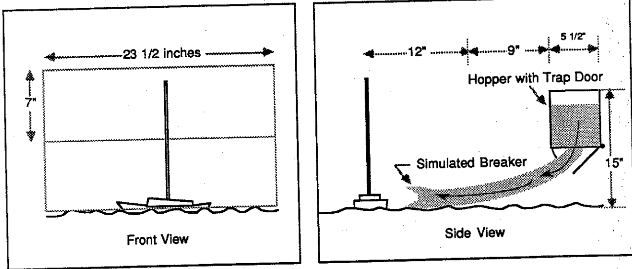
FIGURE 2. Breaking Wave Simulator
