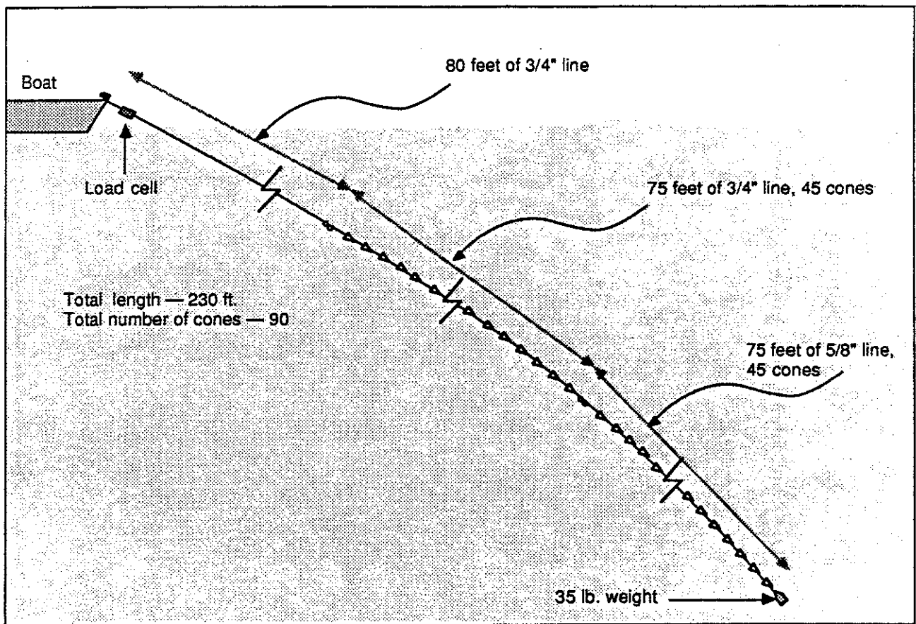
FIGURE 16. Series Drogue
