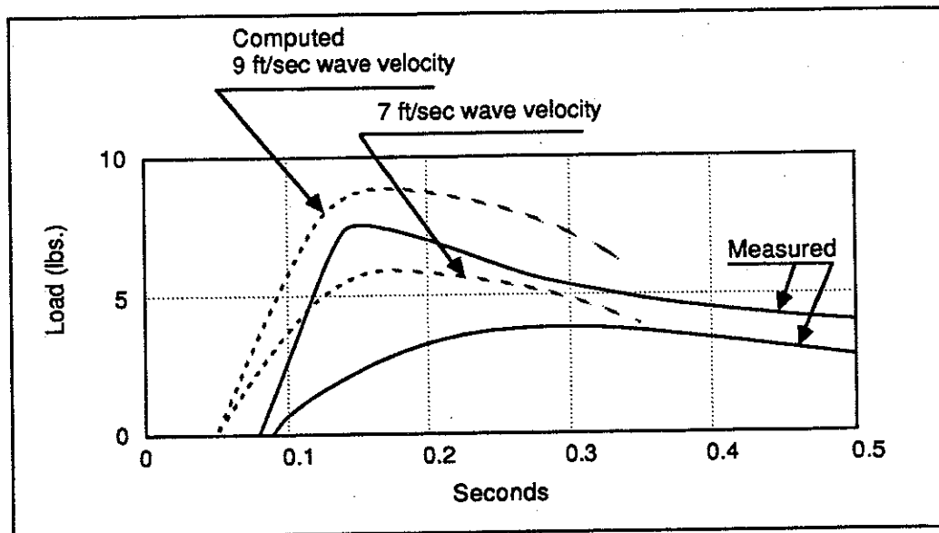
FIGURE 6. Drogue Loads
