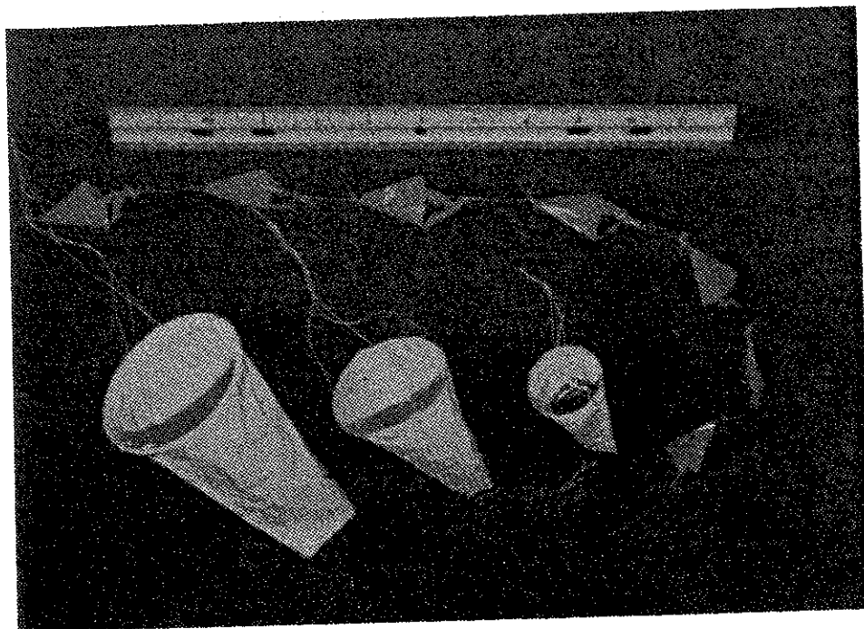
FIGURE 8. Drogue Models
